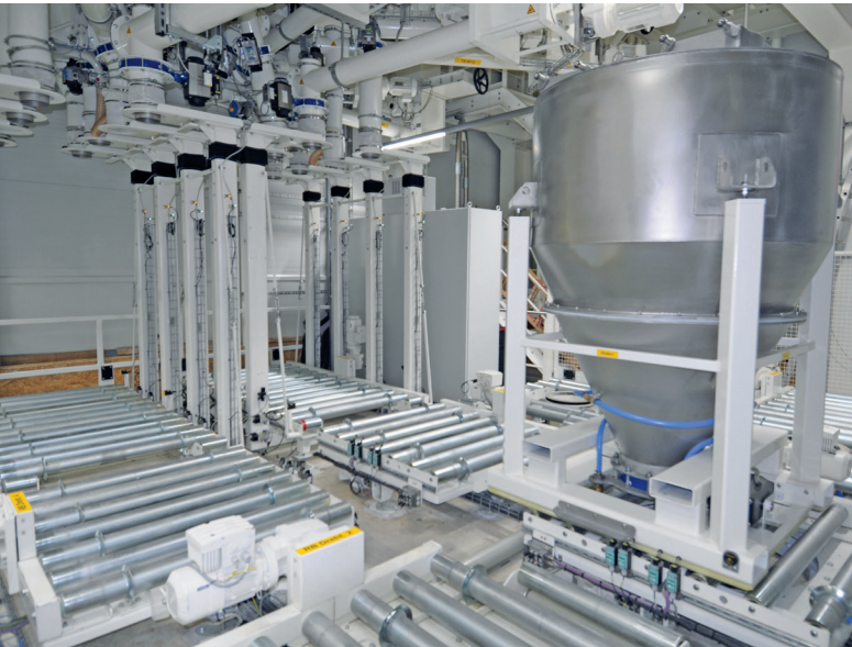
Transport via robust roller conveyor system with turntable
